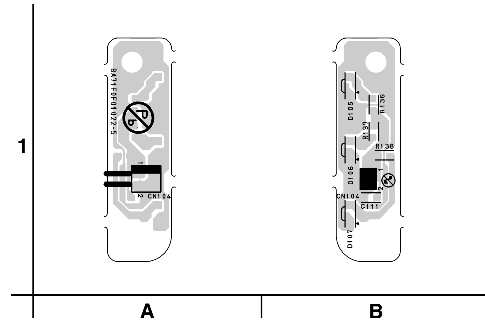
LED CBA Top & Bottom View
