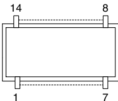
BA10324AF-E2
